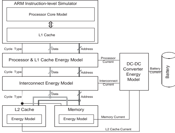
Figure 1: Simulator Architecture
