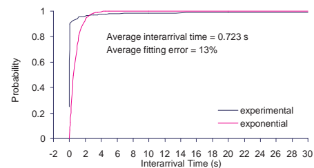
Figure 2: User request arrivals in active state for hard disk
