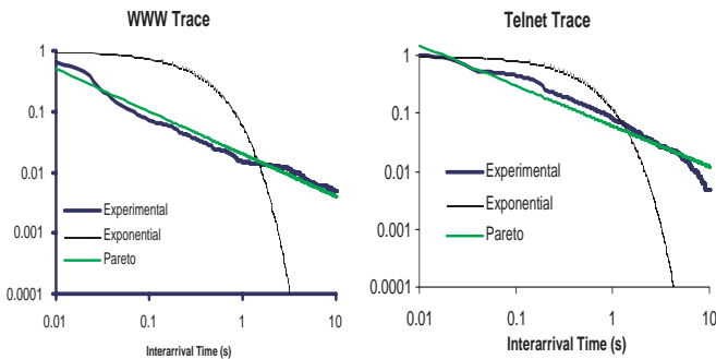
Figure 4: WLAN idle state arrival tail distribution
