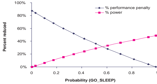
Figure 10: SmartBadge DPM results
