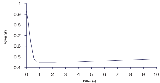
Figure 13: Hard disk power consumption vs. filtering time
